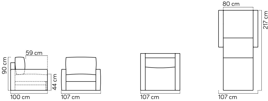
423P - Big chair bed Puma
